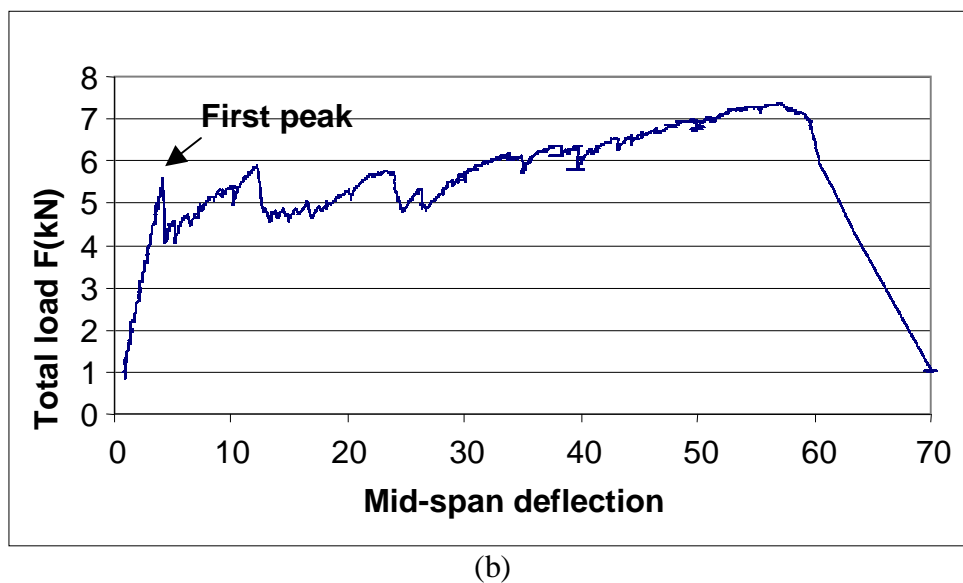
Fig.12. Typical out-of-plane bending test results
