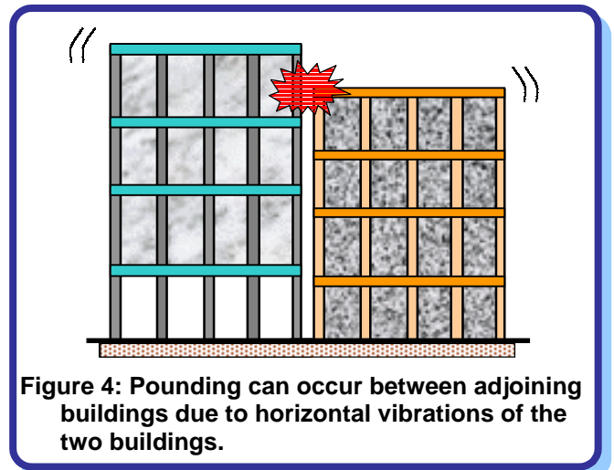
Figure 4: Pounding can occur between adjoining buildings due to horizontal vibrations of the two buildings.
